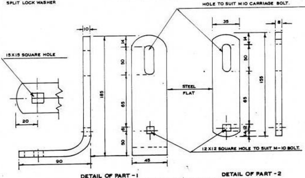
FIG.2:- MOUNTING DETAILS OF 11KV FUSE CUTOUT
